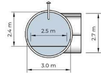
Exterior side
