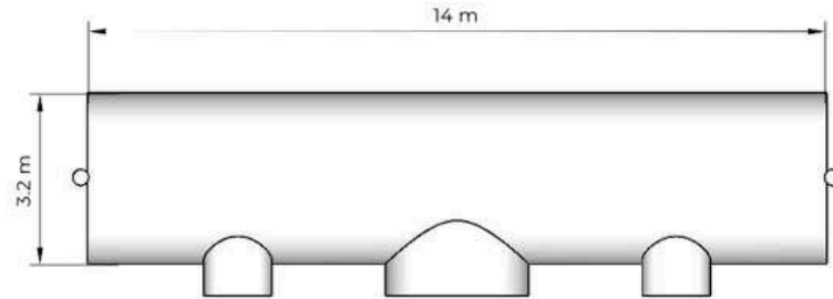
Exterior plan
