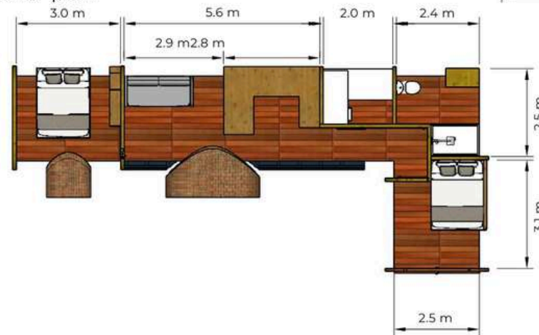
Interior plan
